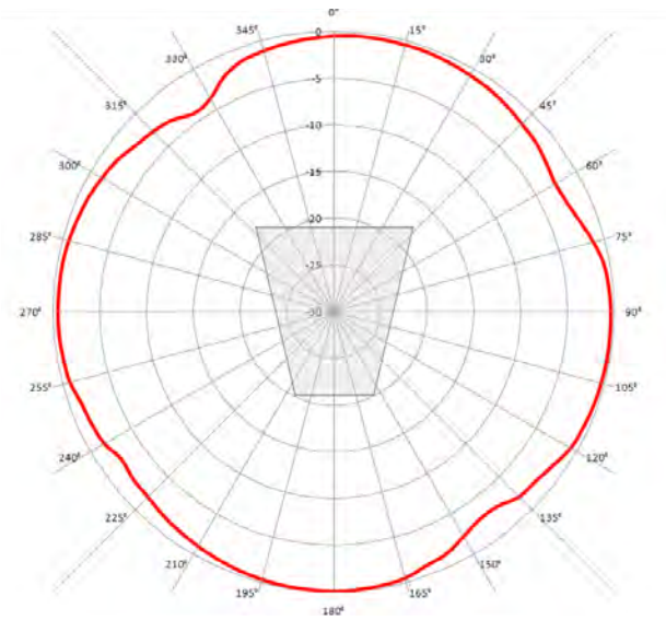
Microphone Array Voice Bandwidth Pickup Polar Pattern
